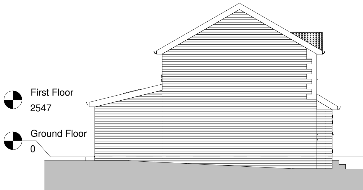
Left Elevation 1 : 100
