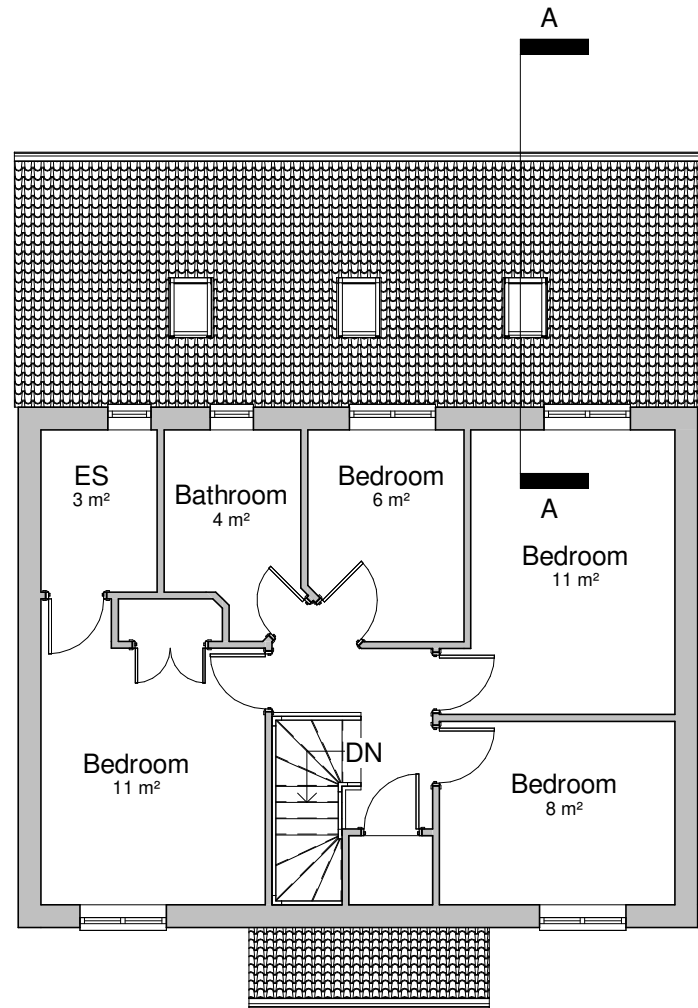
First Floor 1 : 100
