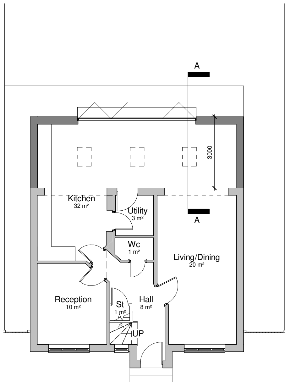
Ground Floor 1 : 100
